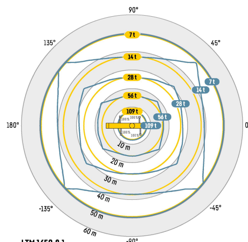
54 m 100% 360° 66 t
